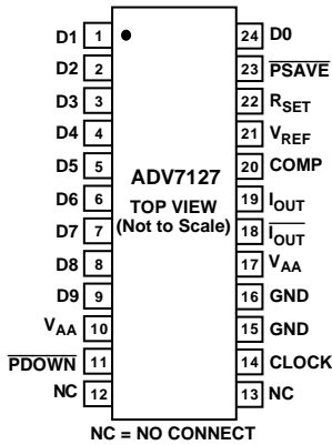
24-Lead TSSOP
